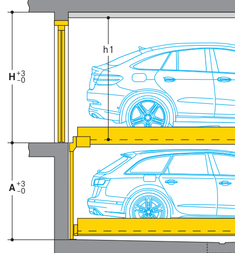
Combilift 542-230
